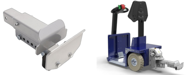
Adjustable hitch for Roll box
